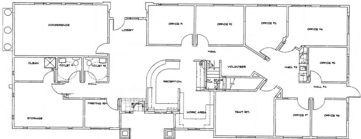
NORTH FIRST FLOOR PLAN SCALE: 1/4" = 1' - 0"
