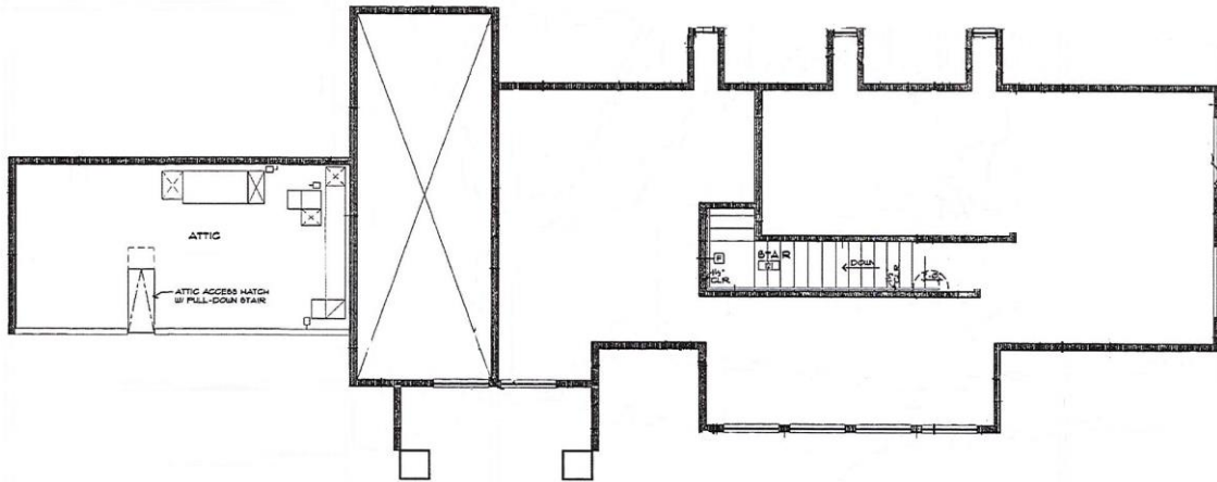
NORTH SECOND FLOOR PLAN SCALE: 1/4" = 1' - 0"
