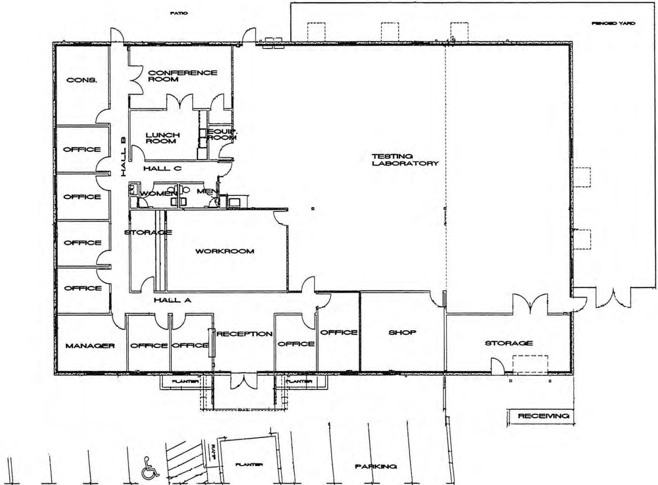
FLOOR PLAN
