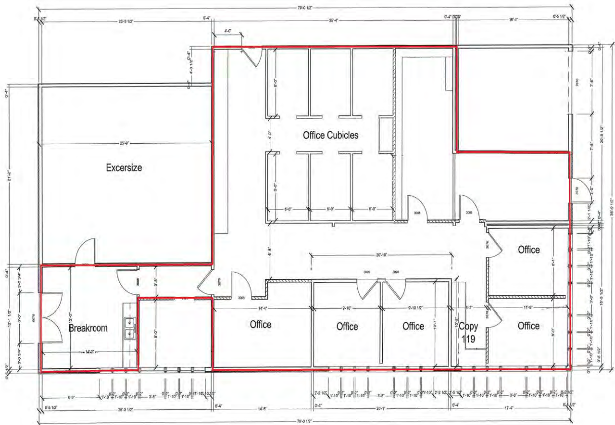
A NEW FIRST FLOOR PLAN SCALE: 1/8"=1'-0"
